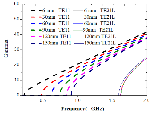
Fig. 4 The propagation constants of TE11 mode and TE21L mode in QRWG with different gap width g .
