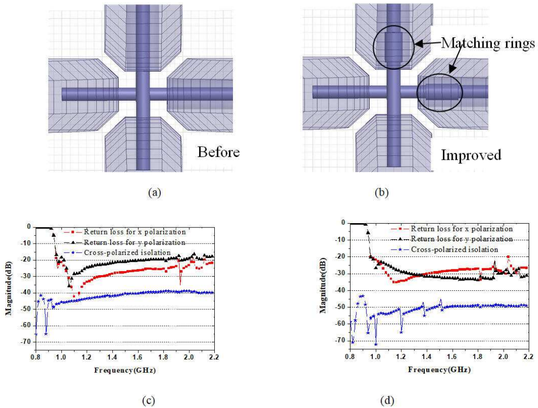
Fig. 7 (a) Structure of original OMT with normal probes. (b) Structure of improved OMT with matching rings into the probes. (c) Full wave simulation of two orthogonal polarization ports for original OMT. (d) Full wave simulation of two orthogonal polarization ports for improved OMT.
